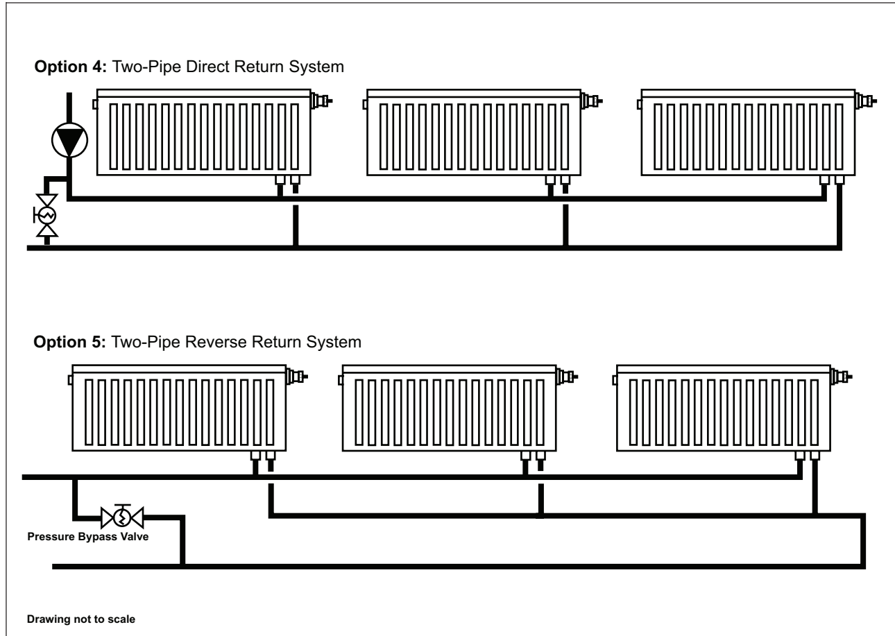
Fig. 12 Two-pipe System Options
